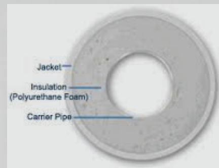
Cross Section - Pre insulated Pipe
